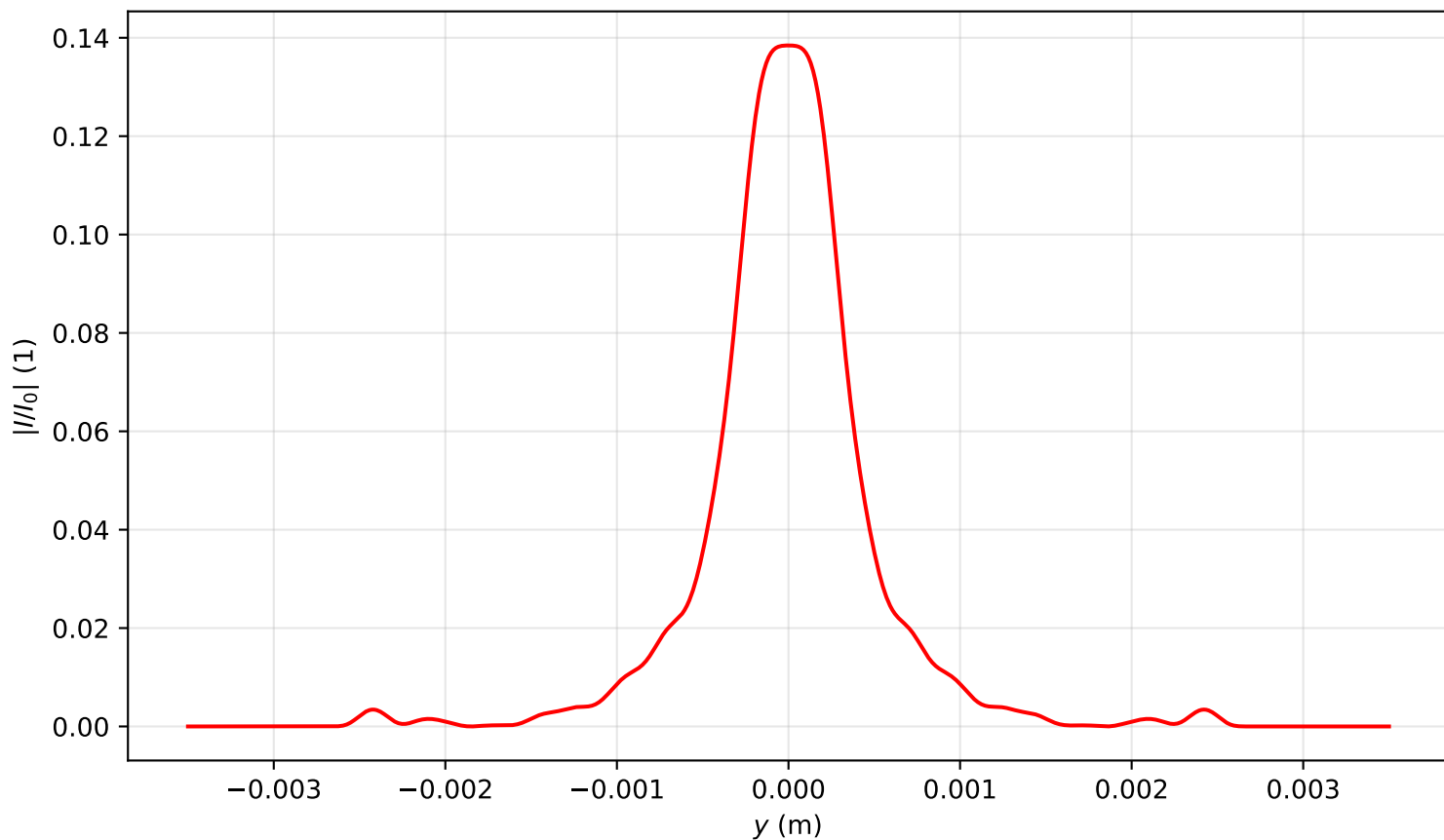
Intensity profile I(x=0, y, z=3.344)/I_0 , P_{in}=5.0P_{cr} , artificial time
